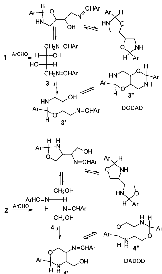
Scheme 1. All possible products (diimines, mono- and diacetals) from the reaction of threo -1,4- and threo -2,3-diaminobutanediols ( 1 , 2 ) with aromatic aldehydes; the six-membered bicyclic systems are the cis -dioxadiazadecalins (DODAD) and cis -diazadioxadecalins (DADOD).
